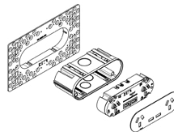
ADJUSTABLE MOUNTING ASSEMBLY
